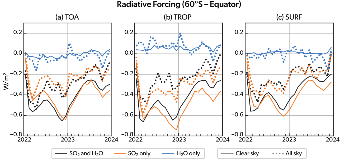
Figure 7.3: All-sky (dotted curves) and clear-sky (solid curves) (0-60°S) average net SA+WV, WV, and SA IRFs ( \text{W m}^{-2} ) from the WACCM6MAM-nd run with nudged meteorology: (a) at TOA; (b) at TROP; (c) at SURF. (Adapted from Quaglia et al., 2025.)
