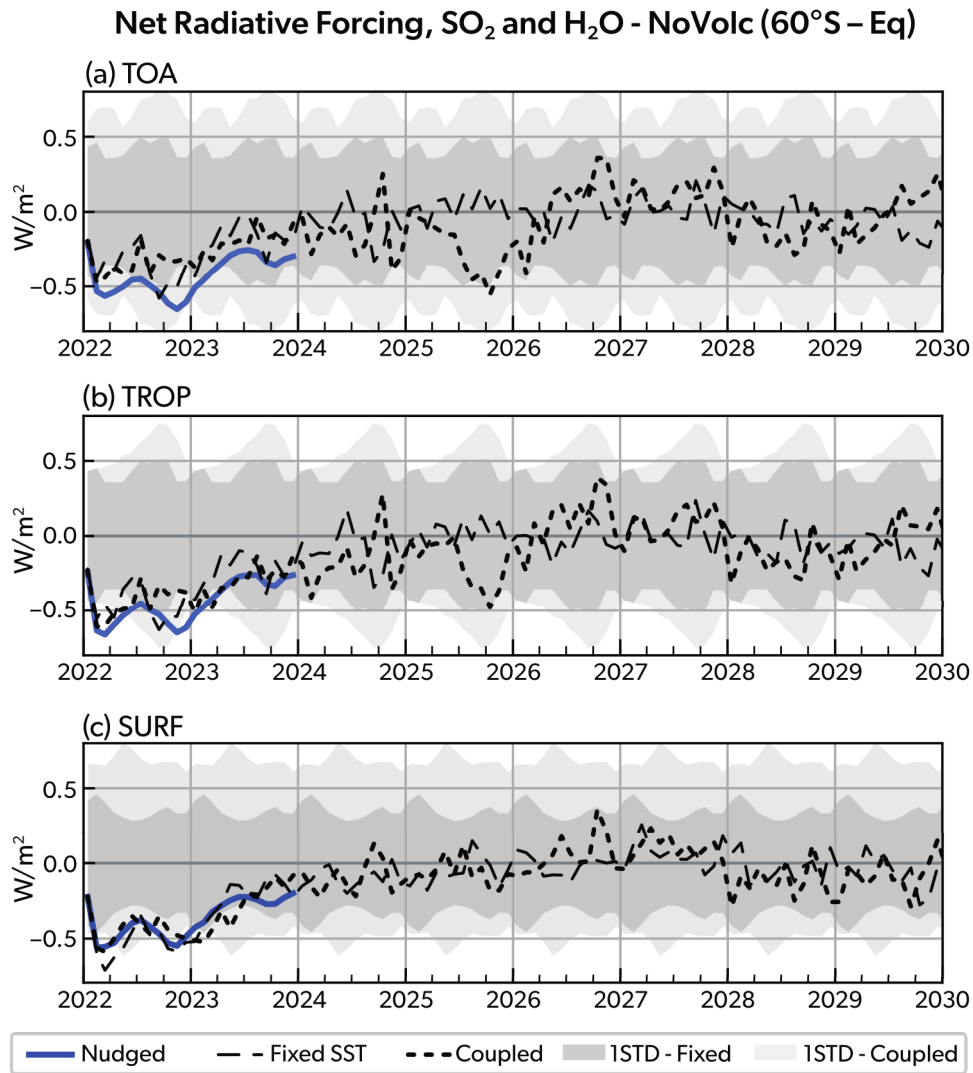
Figure 7.6: Near-hemispheric (0–60°S) SA+ WV clear-sky RFs ( W\ m^{-2} ) from the WACCM6MAM-nd run with nudged meteorology, the WACCM6MAM-co ensembles with coupled ocean, and the WACCM6MAM-fs ensembles with prescribed SSTs, shown at (a) TOA, (b) TROP, and (c) SURF. Dark shading indicates the one-standard-deviation range for WACCM6MAM-fs, while light shading indicates the one-standard-deviation range for WACCM6MAM-co. (Adapted from Quaglia et al., 2025.)
