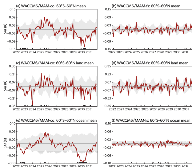
Figure 7.8: Near-global (60°S–60°N) averaged ensemble mean surface air temperature SAT (K) change (Hunga – control) from the WACCM6MAM-co (left column) and prescribed SST WACCM6MAM-fs (right column) ensembles. Red solid lines show the 30-member ensemble mean. Gray shading belts are \pm 2 SAT standard deviations from the control run. (a, b) \Delta SAT_G (global), (c, d) \Delta SAT_L (land), and (e, f) \Delta SAT_O (ocean). Dots at the bottom of the panels indicate the time periods when the SAT perturbation exceeds 2 standard deviations.
