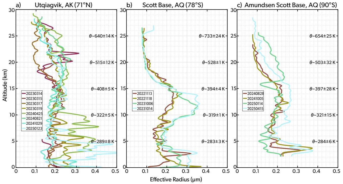
Figure 3.10: Aerosol effective radius derived from balloon sounding measurements (radius range 0.07–1.25 \mu\text{m} ) at polar stations: (a) Utqiagvik (71°N), (b) Scott Base (78°S), and (c) South Pole (90°S). Potential-temperature equivalent levels averaged over the plotted profiles are displayed on the right axis of each panel.
