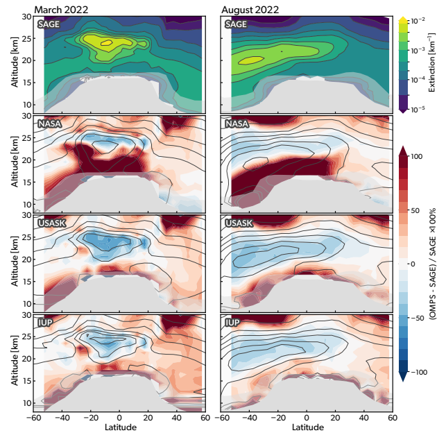
Figure 3.13: Comparison of aerosol extinction at 750 nm from all three OMPS-LP retrievals and SAGE III/ISS. Panels show zonal averages from each instrument and the corresponding percent difference of OMPS-LP from SAGE III/ISS. Black contours show the extinction from each instrument, delineating the region of the Hunga aerosol. Light-grey regions indicate altitudes that are sometimes in the stratosphere; opaque-grey regions indicate altitudes always in the troposphere.
